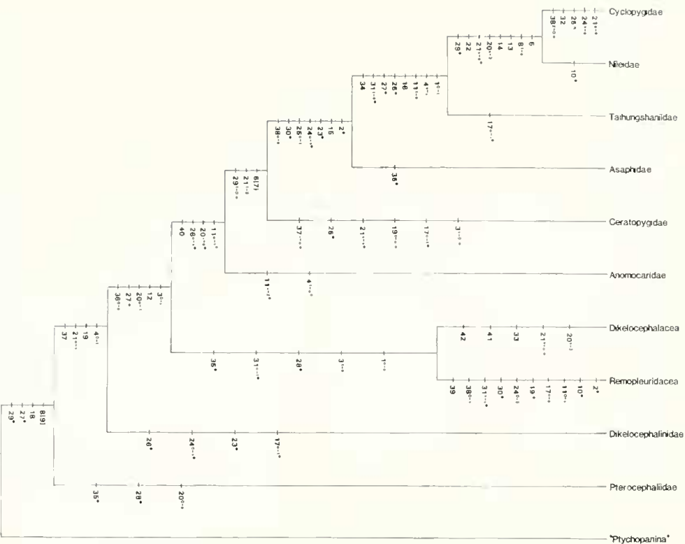
TEXT-FIG. 2. Cladogram produced from the PAUP computer analysis of the characters given in Table 2. Another equally parsimonious cladogram is shown in text-fig. 3. Note that text-figs 2 and 3 resemble each other apart from the position of Dikelocephalidae and Pteroccephalidae . Pteroccephalidae and Anomocaridae are coded separately (cf. text-fig. 1) rather than included in Anomocaridae sensu lato . Numbering of Characters as in Table 2. Direction of character transformation for multistate characters is indicated. For symbols see text-fig. 3.
